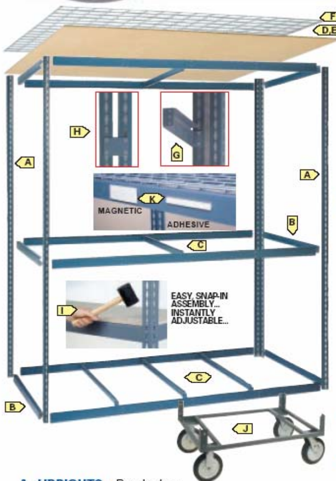
ANGLE POST 2 1/4" x 1 1/2"
