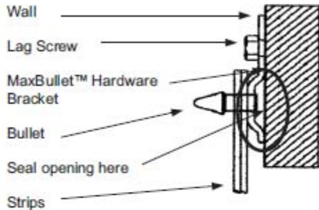
Diagram 1 Side View
